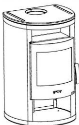
JAVA
